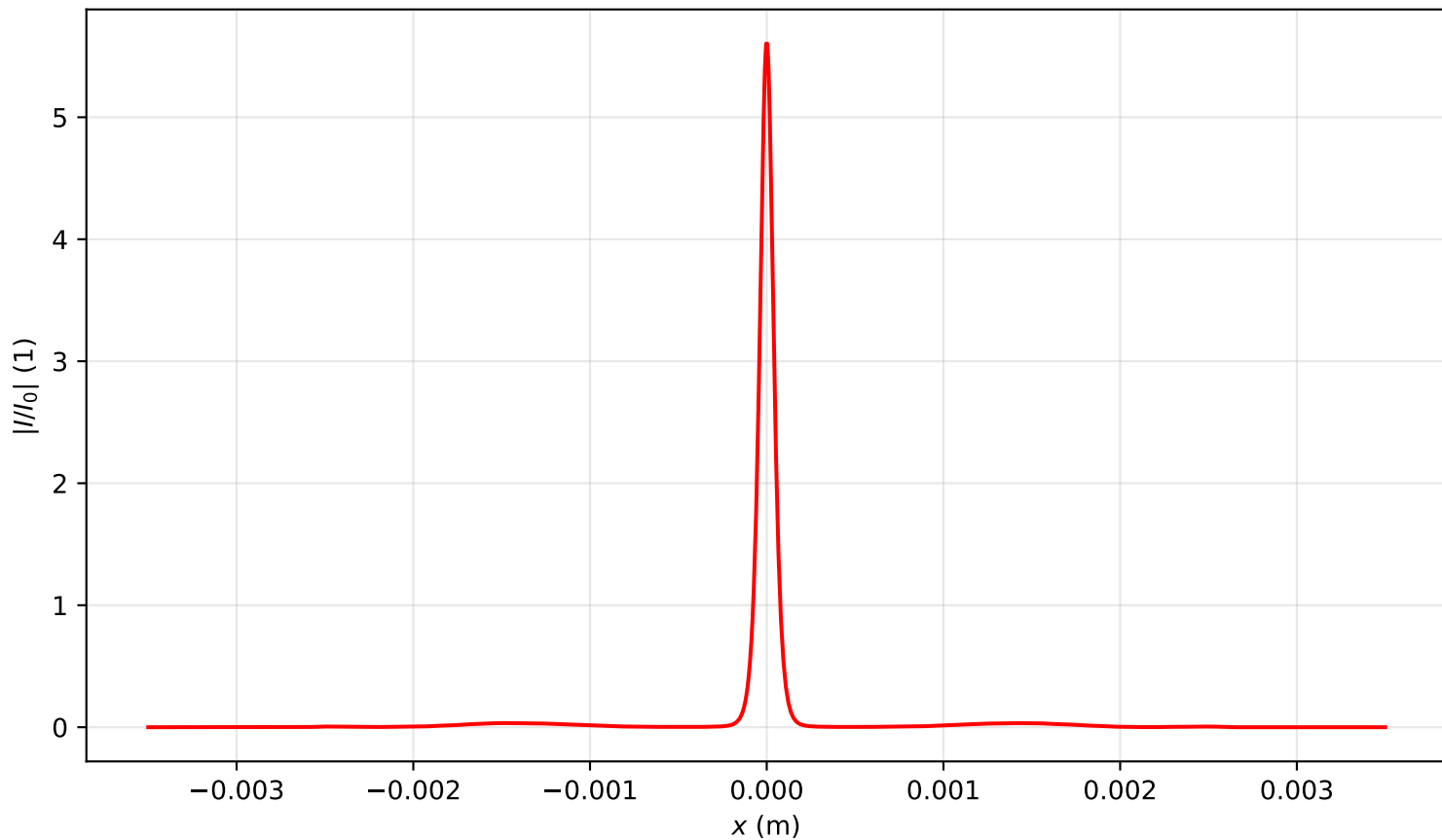
Intensity profile I(x, y = 0, z = 1.115)/I_0 , P_{in}=7.0P_{cr} , artificial time
